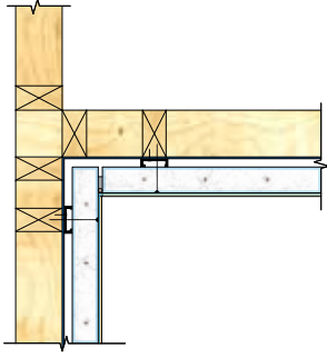
5. Internal Corner - Page 42
