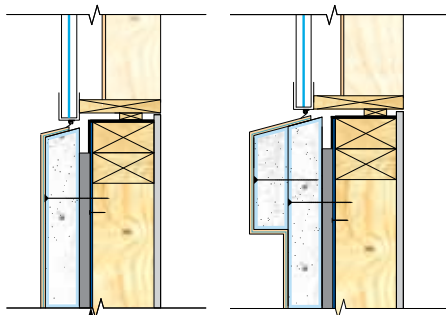
7. Window Sill - Page 43
