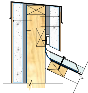
8. Parapet Detail - Page 47
