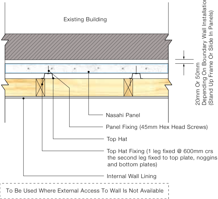
DETAIL 12.2 - Boundary Wall Fixing Detail A
