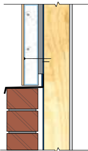
7. Cladding to Brick Detail - Page 45
