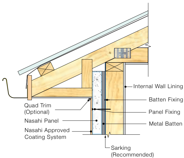
DETAIL 4.3 - Eave Detail (Panel Flush With Lining)
