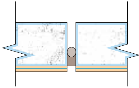
1. Control Joint - Page 47
