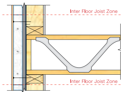
3. Internal Floor Junction - Page 46
