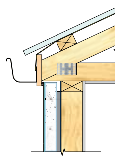
6. Flush Eave - Page 44
